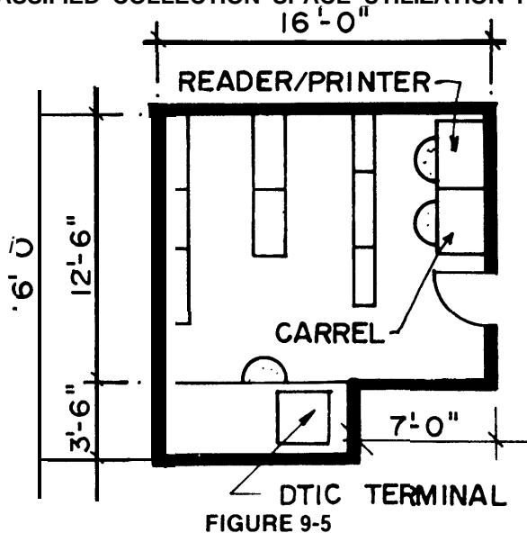
CLASSIFIED COLLECTION SPACE UTILIZATION PLAN
